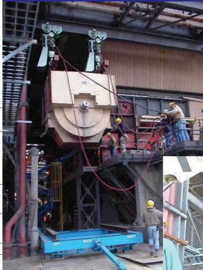
Photos show maintenance of ID fan & rotor at a local power plant
